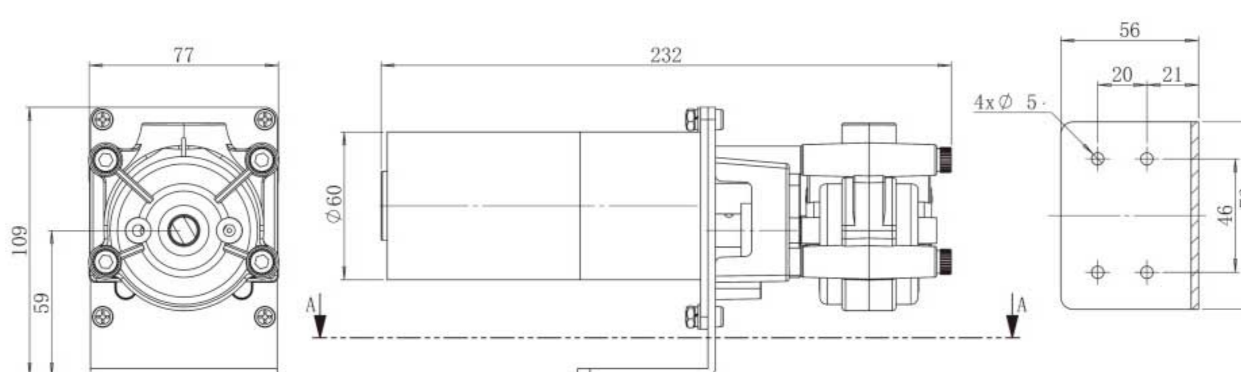
Dimension Drawing(Unit: mm)
