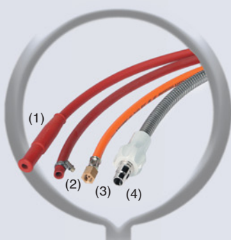
DVGW-Safety tubing (1) for push-fit connection (0.5 m) Art.-No. 6.000.102 (2) for push-fit connection, with 2 tubing clips (0.5 m) Art.-No. 6.000.101 (3) for threaded connection (0.5 m) Art.-No. 6.000.112 (4) for gas socket connection (0.5 m) Art.-No. 6.000.122 other length on demand
