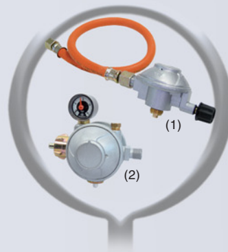
(1) Safety adapter R with pressure regulator and DVGW- tubing (0.5 m) for gas cylinders R 901 / R 904 / R 907 Art.-No. 6.000.840 (2) DVGW low press. regulator DIN 4811-4, for household liquid gas installation, with overpress.-, temperature- fuse & manometer, for gas bottles up to 14 kg Art.-No. 6.000.150
